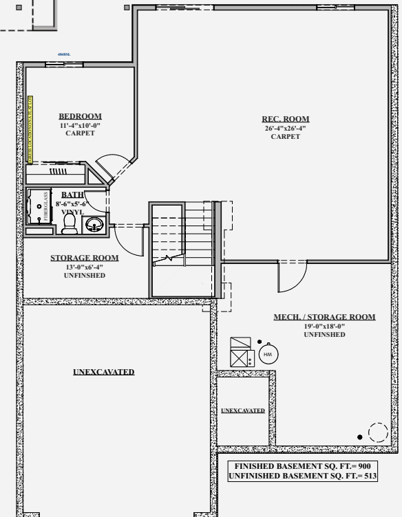
FINISHED BASEMENT/ FOUNDATION PLAN
